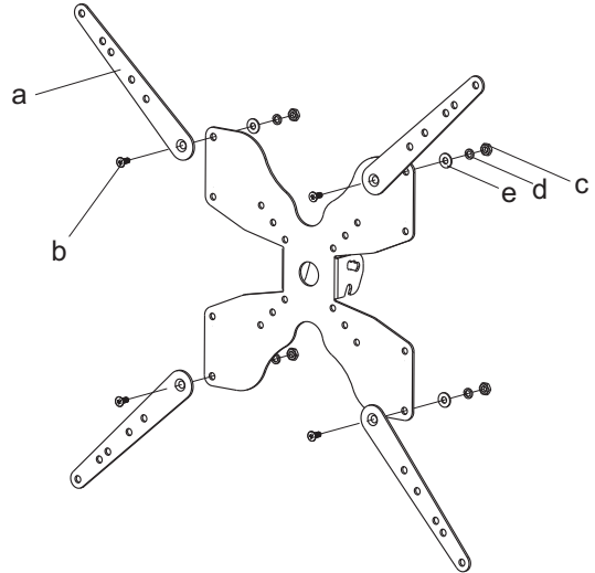
(4)Washer-e
